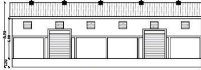
ELEVATION SCALE 1:100
