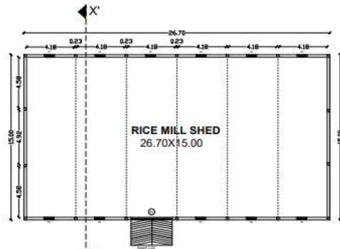
PROPOSED RICE MILL SHED PLAN SCALE 1:100
