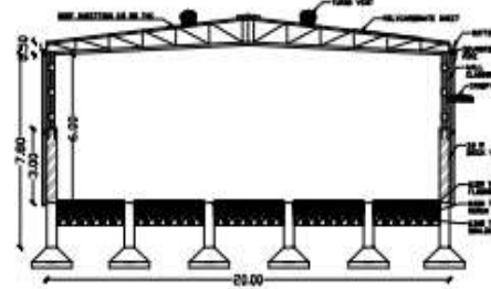
SECTION X-X' SCALE 1:100
