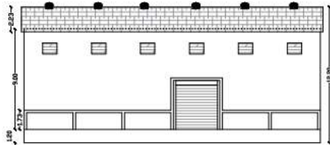
ELEVATION SCALE 1:100
